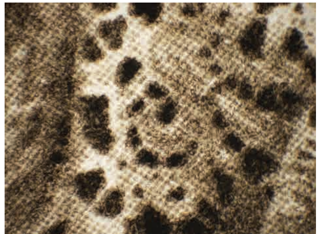
Figure 19b Detail of the print in fig. 18 (25x magnification), showing a high-definition rotogravure pattern.
