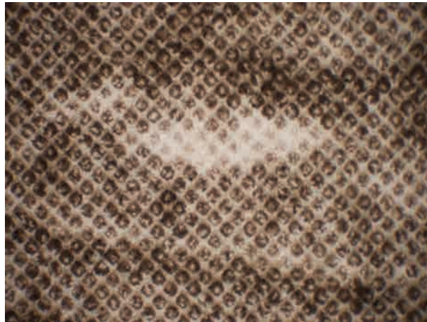
Figure 10a Microscopic pattern of a typical rotogravure print (10x magnification).
