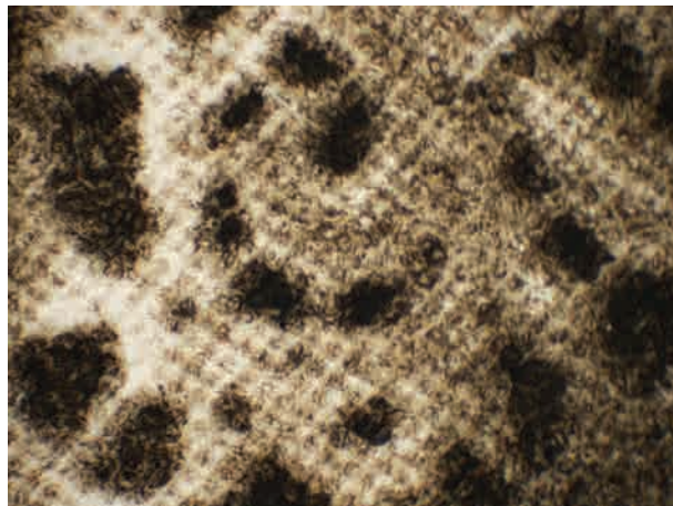
Figure 19c Detail of the print in fig. 18 (40x magnification), showing a high-definition rotogravure pattern.
